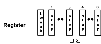
Fig. 6. Pipeline register in Luffa_negative technique
