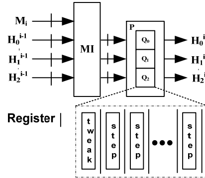
Fig. 5. Pipeline registers in Luffa_positive technique
